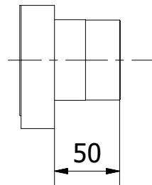
F1-F4 & B1-B4 RG 1"/1 1/4" THREADED PIPE
