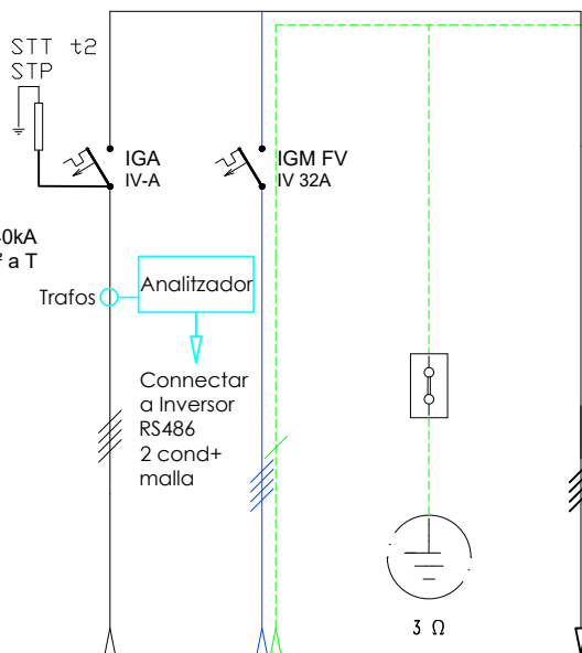
QGCP - Quadre General Com. i Prot.
